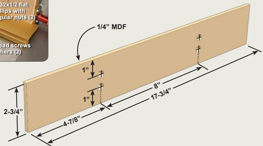
Fig. 11 Backing Board Dimensions
